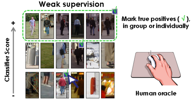
Figure 2. Detections are presented to the oracle ordered by classifier score and in CW size. The oracle marks right detections individually or in groups indicated by initial and final clicks.
