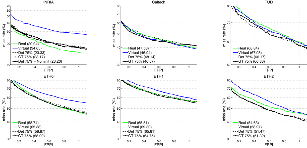
Figure 4. Miss rate vs FPPI curves with the maximum amount of validated detections ('Det' 75%) and corresponding manually annotated BBs ('GT' 75%) from INRIA training set, for different testing sets. 'Real' stands for the case of training with the full INRIA training set, while 'Virtual' refers to training with the virtual-world data. The number in parenthesis is the average miss rate (%) of the respective curve.
