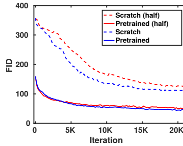
Fig. 6: Model capacity
