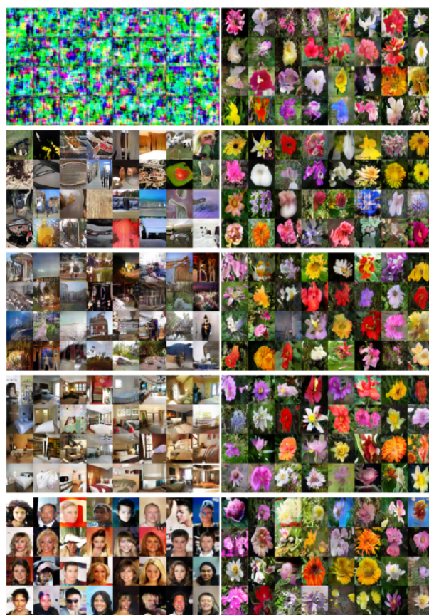
Fig. 7: Images sampled from each of the source models (left) and after fine tuning 5K iterations with Flowers (right). From top to bottom: from scratch, ImageNet, Places, LSUN bedrooms, CelebA.
