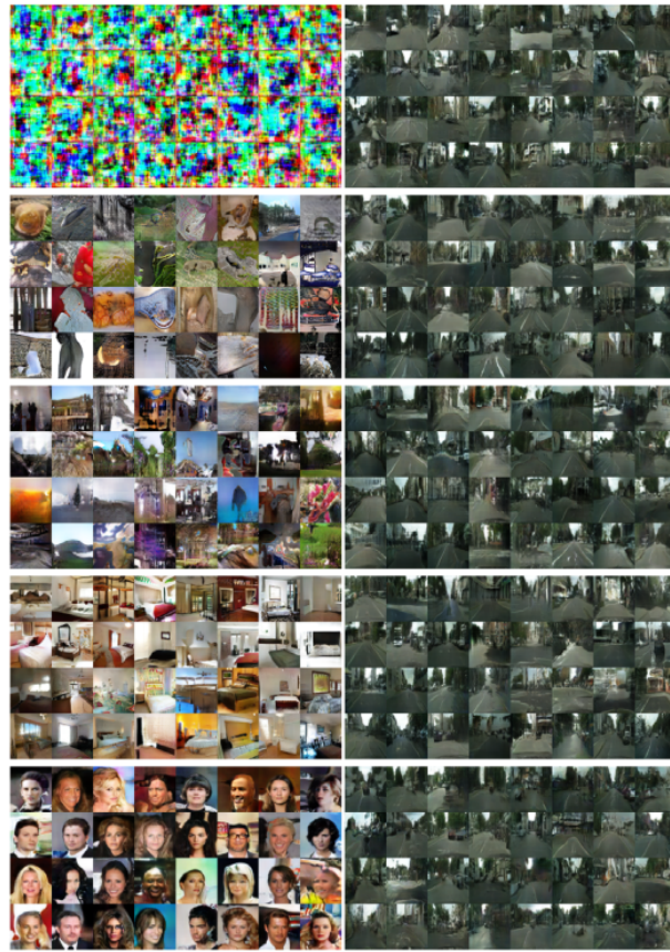
Fig. 10: Images sampled from each of the source models (left) and after fine tuning 5K iterations with Cityscapes (right). From top to bottom: from scratch, ImageNet, Places, LSUN bedrooms, CelebA.
