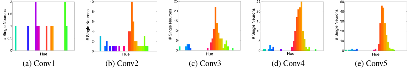
Figure 4: Number of single color neurons per hue for the five convolutional layers. Shallower layers (conv1 and conv2) present a more equitable distribution along the hue dimension. Deeper layers (conv3, conv4 and conv5) concentrate single neurons on Orangish and Bluish regions following the color bias of the training dataset.
