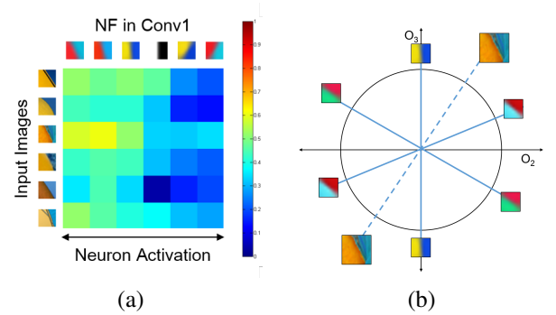
Figure 6: Orange-blue edge representation in Conv1. (a) Activation values of some neurons in Conv1 (NFs are in first row) to a set of images (first column) in a color scale from blue (minimum) to red (maximum). (b) Double neurons in Conv1 over the hue space. Orange-Blue image (dashed line) is represented between two main neurons in Conv1 (Blue-Yellow and Red-Cyan).
