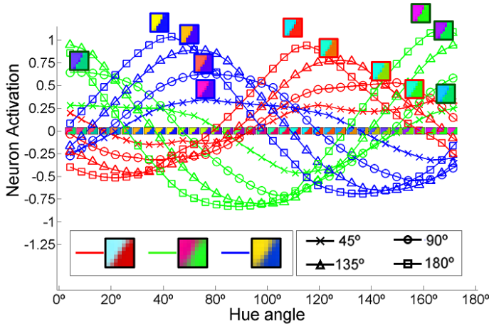
Figure 5: Representation of color edges. Activation curves of three different double opponent color neurons at Conv1 to 4 different types of edges regarding the opponency property of the pair of colors on the tested edges: opponent edges (180), 135, 90 and 45 color edges.
