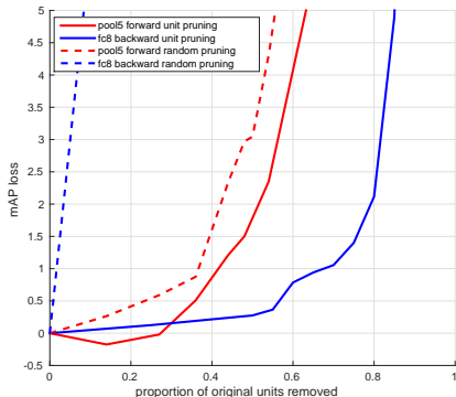
Figure 2: Performance loss as a function of parameter reduction.
