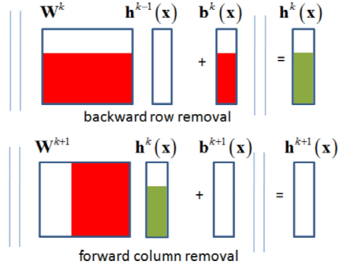
Figure 1: Example of backward and forward unit pruning. We use \|\cdot\| to indicate the \text{relu}(\cdot) activation function. Based on knowledge that some unit activations \mathbf{h}^k(\mathbf{x}) are zero (indicated in green), we can reduce the parameters of \mathbf{W}^k , \mathbf{W}^{k+1} and \mathbf{b}^k (indicated in red).
