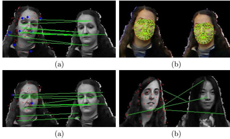
Fig. 2. Face identification analysis. Red dots: SURF candidate keypoints not matched based on descriptor distance. Blue dots: candidate keypoints discarded as outliers using RANSAC based on mesh transformation criteria. Green line: final matches considered for identification. (a) Example of images not aligned after face detection and background removal. Several outliers are detected using RANSAC (blue dots), reducing final identification probability of being the same user category (71.4% of probability in this example). (b) Shows the intermediate results of applying ASM meshes to both faces before alignment. (c) Applying the whole proposed process. Now the probability of identification increases up to 98.4%. (d) An example of alignment and identification for two different categories, with a result of 32.3% of probability.
