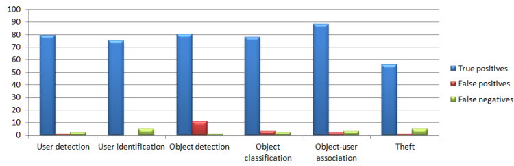
Fig. 4. Mean surveillance system performance
