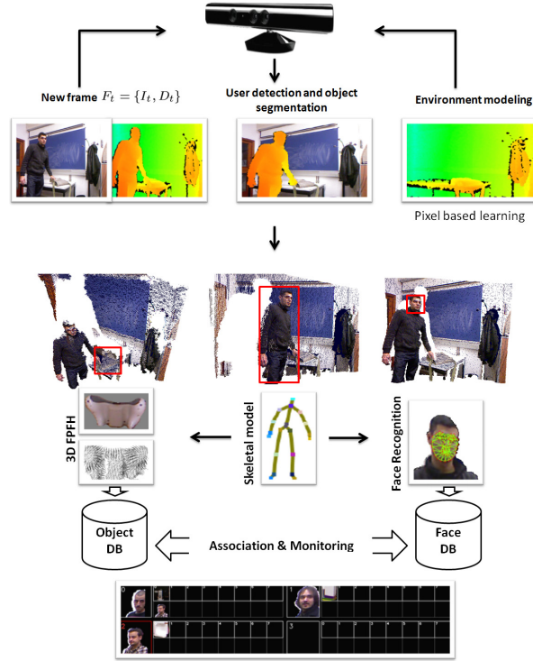
Fig. 1. Multi-modal user identification and object recognition surveillance system
